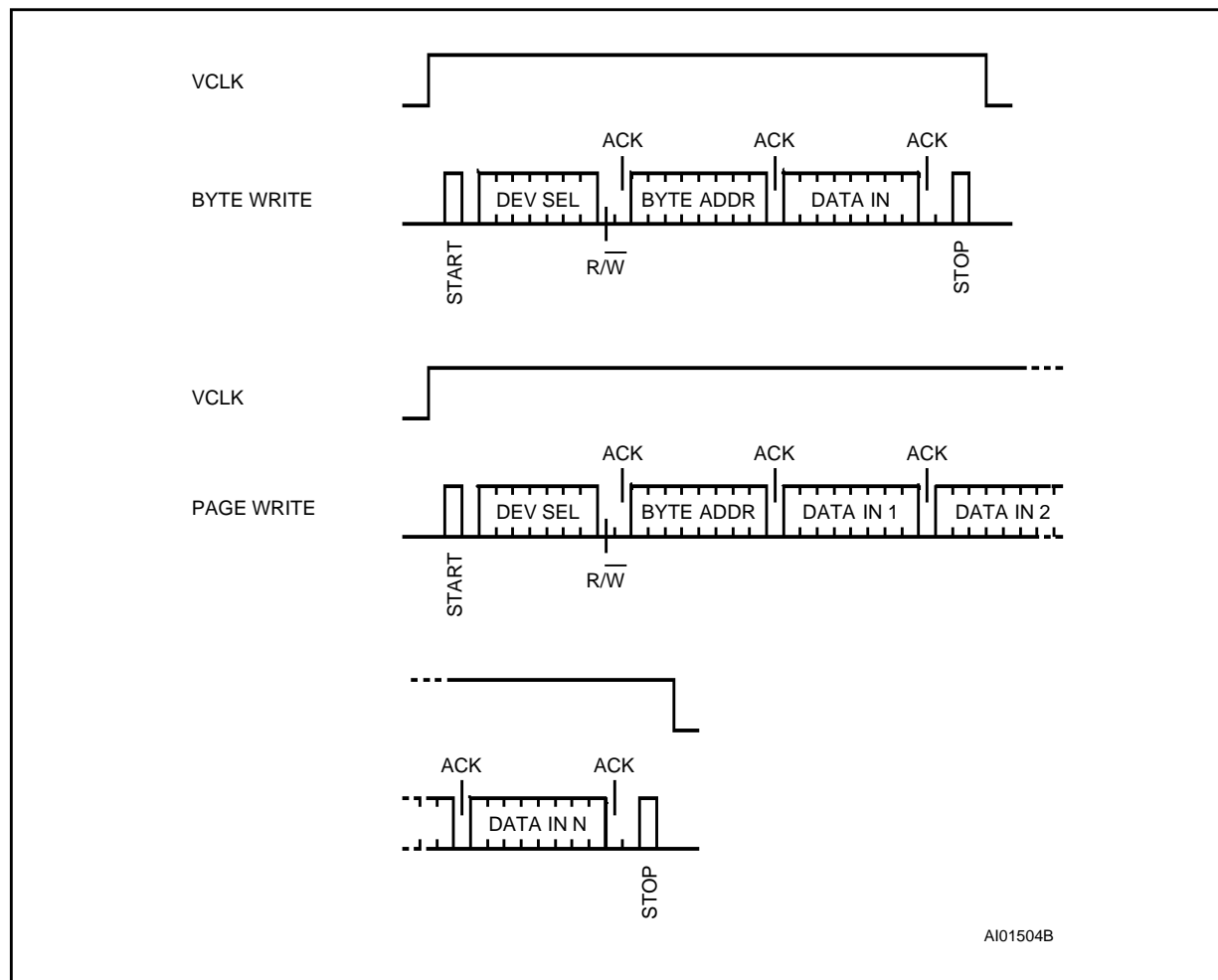
Figure 10. Write Modes Sequence
