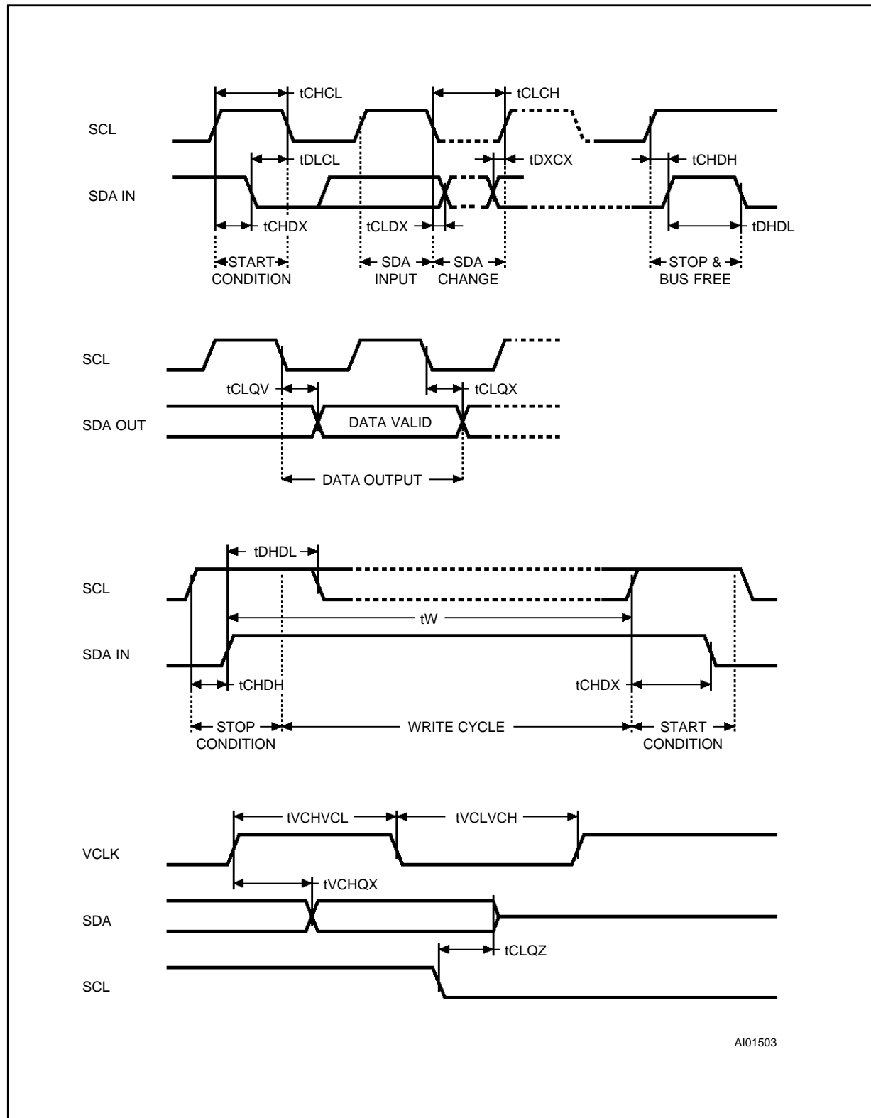
Figure 6. AC Waveforms
